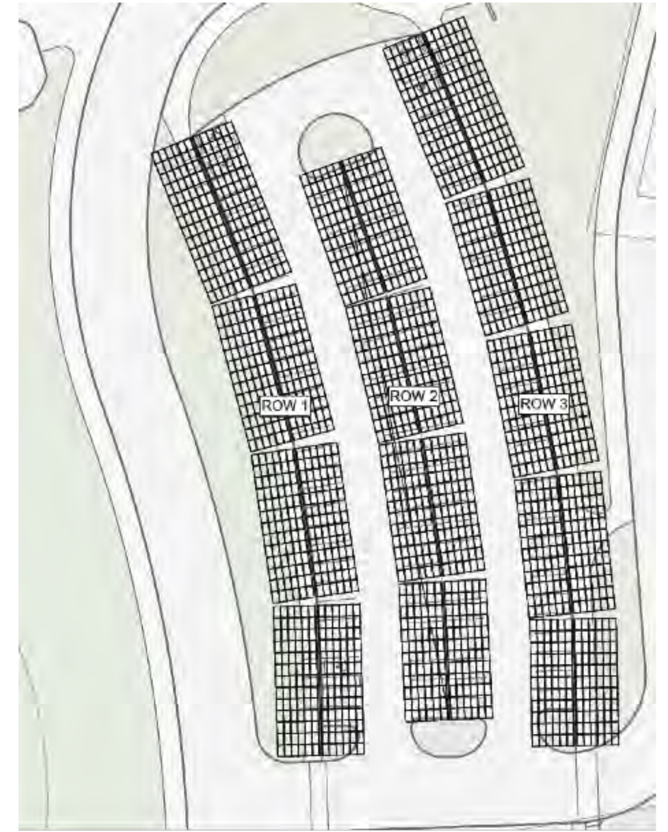
V-Tilt Canopy, Expanded
